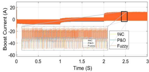
Fig. 3. Boost Current
