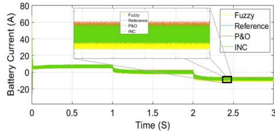
Fig. 5. Battery Current
