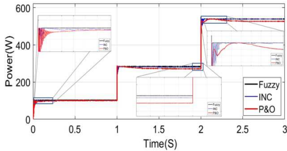
Fig. 7. Panel Power
