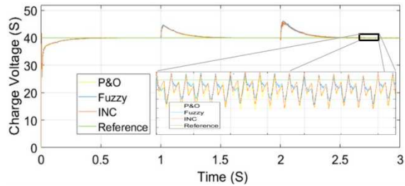
Fig. 4. Charge Voltage
